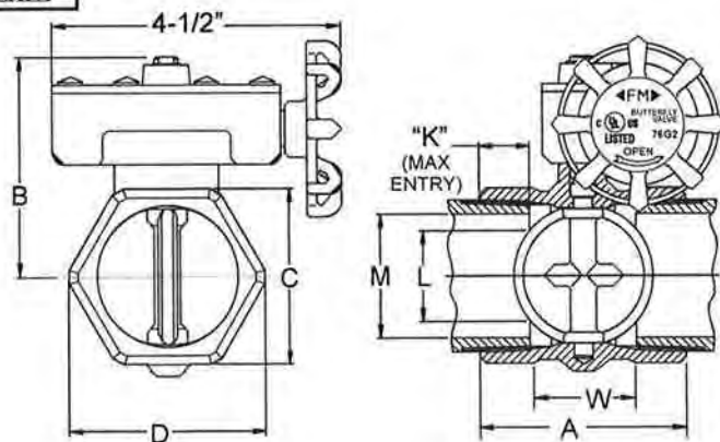
BB-SC100 Sizes 1", 1-1/4", 1-1/2", 2", 2-1/2"
