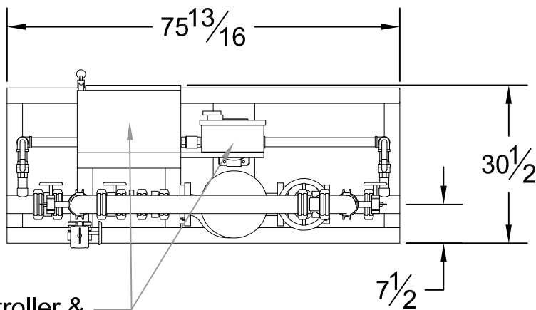
Main Controller & Jockey Controller
